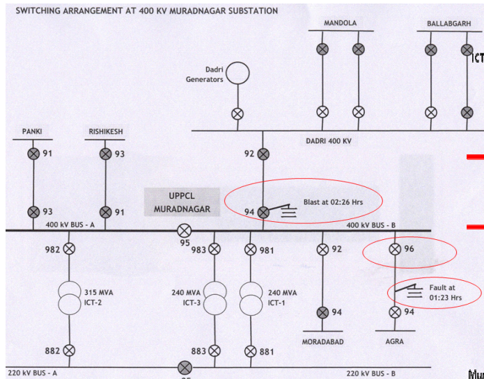
Figure 2: 400 kV Muradnagar schematic
