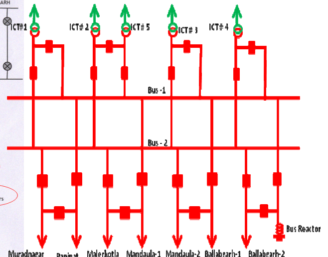
Figure 3: 400 kV Dadri switching diagram
