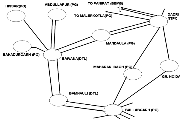
Figure 4: Sketch of 400 kV Delhi ring main system
