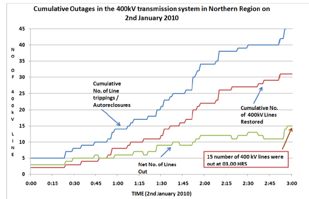
Figure 5: Cumulative number of lines tripped or restored during 0000 to 0300 hrs of 02nd Jan-2010
