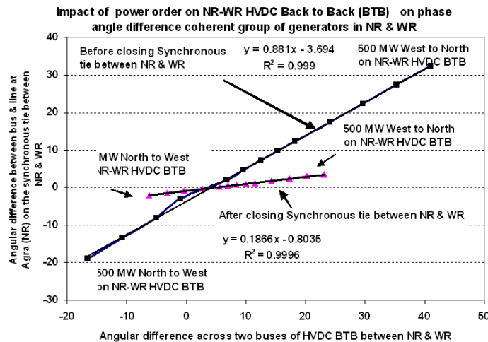
Figure 4 Simulation Results for energisation of synchronous link between NR & WR
