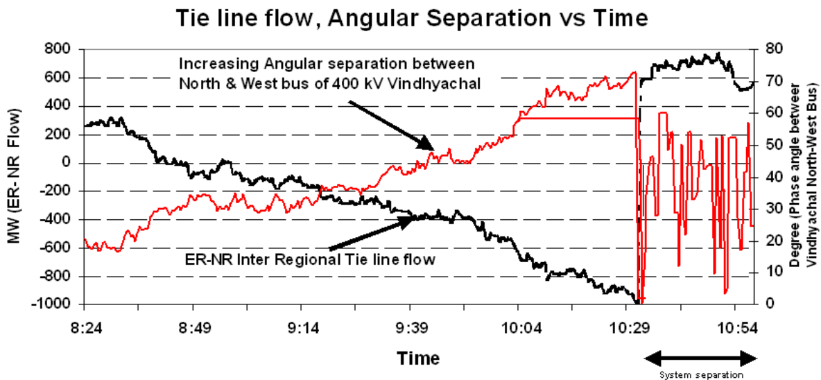
Figure 3 Phase angle trend before and after system separation in NEW grid on 22nd Oct 2006
