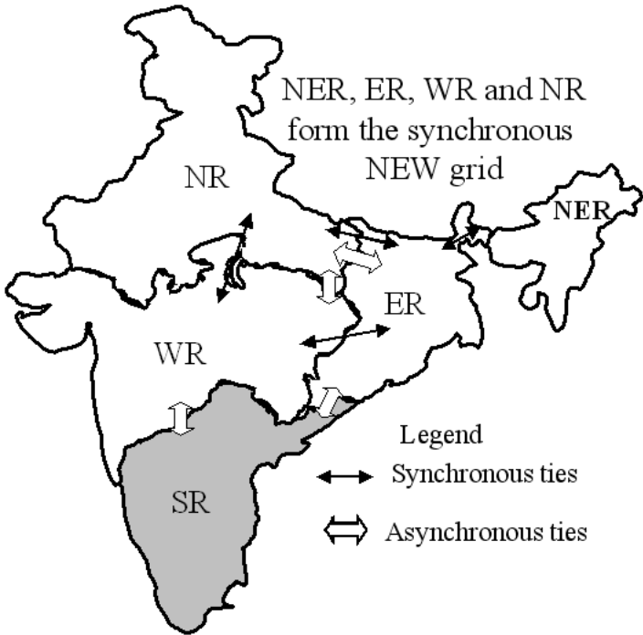
Figure 1: Two synchronous power systems in India
