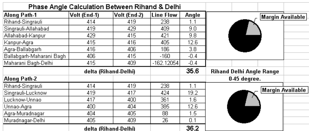
Figure 2 Phase Angle Calculation at Control Center using SCADA measurands
