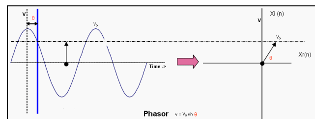
Fig. 1 - Phasor represents magnitude and phase angle at any given instant of sine wave of voltage or current.[2]
