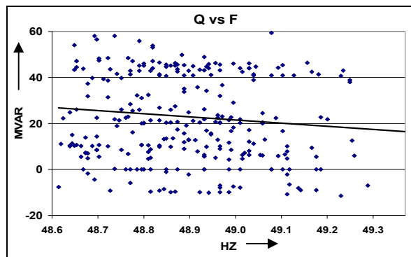
Fig.4.3 Scatter Plot: Freq. Vs MVAR (Radial Load of Okhla)
